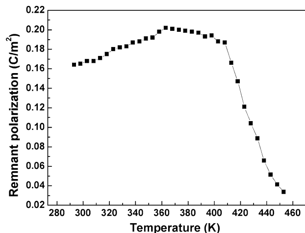
Fig. 3 Temperature dependence of remnant polarization P_r of unpoled PMN–0.3PT single crystal
