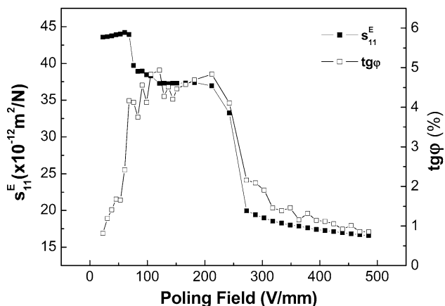
Fig. 5 The elastic compliance s_{11}^E and mechanical loss factor \text{tg}\phi of PMN-0.3PT as a function of poling field measured at 360 K
